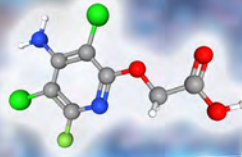
Fluroxypyr
