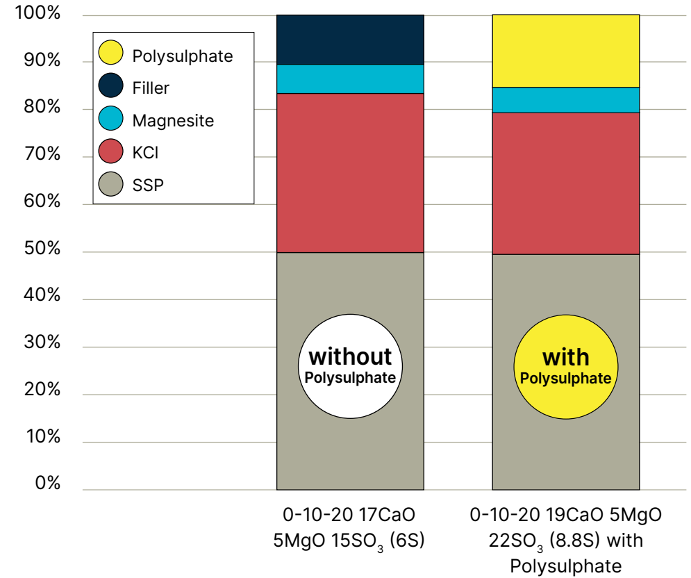
Comparison of PK 0-10-20+5MgO production at ICL plant with Polysulphate and alternative sources
