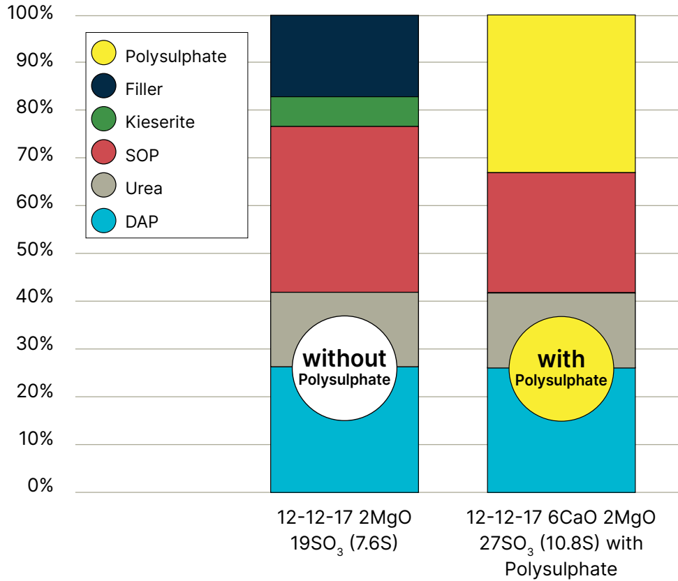
Comparison of NPK 12-12-17+2MgO production with Polysulphate and alternative source
